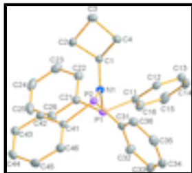
Fig. 1. Molecular structure of the title compound. Displacement ellipsoids are drawn at the 50% probability level.
